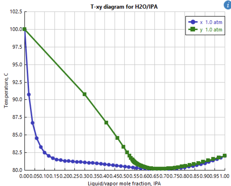
Figure A.8.1.1: T-xy Diagram of IPA & Water
