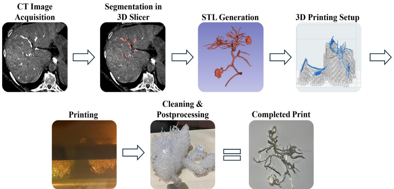
Fig. 2. Flowchart of the model production process: 1) CT scan provided by Dr. John Angle (IR Department at UVA Health). 2) Used automatic thresholding followed by manual adjustment (the vessels identified by the thresholding are highlighted in pink). 3) The segmented, thresholded model is rendered in 3D. 4) The STL file is exported to PreForm 3D printing software; supports are generated (in white) and the printing parameters are adjusted. 5) The SLA printer is prepared, including the tank, resin cartridges, and build plate. The print is allowed to run (~22 hours). 6) Post-processing steps are completed, including an isopropyl alcohol bath (10 minutes), manual removal of supports, and light-curing (20 minutes). 7) The solid model is completed.
