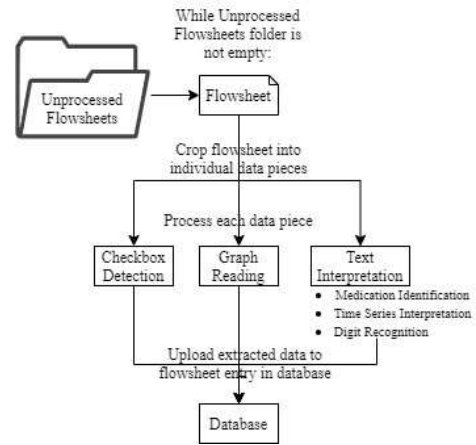
Fig. 5. Integration Diagram
