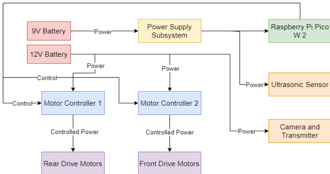
Figure 2: Car Component Layout
