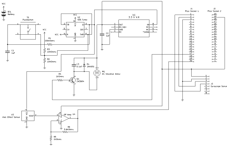
Figure 7: Schematic of Glove PCB.
