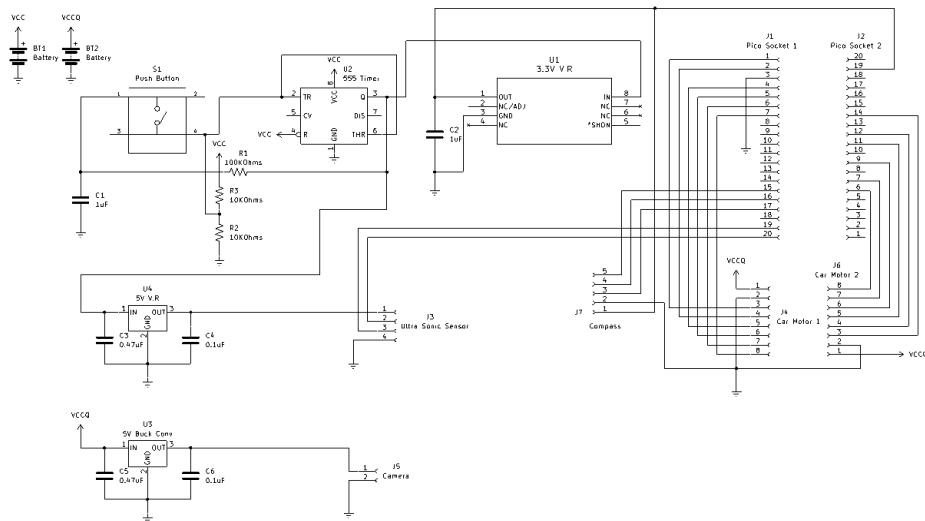
Figure 8: Schematic of Car PCB.
