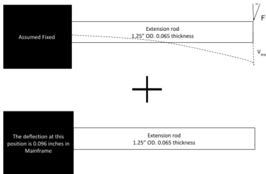
Figure 1B: Superposition approach for corrected deflection
