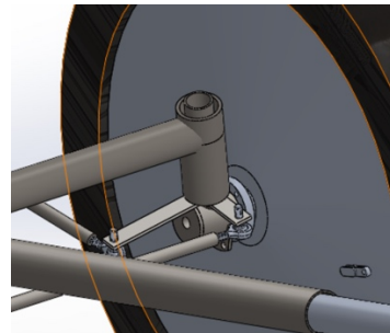
Figure 8b Axle Design and Frame Attachment
