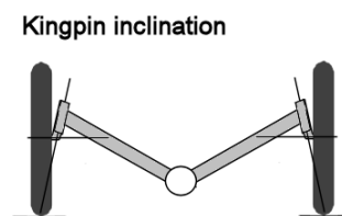
Figure 1: 'Trike with zero scrub radius [8]
