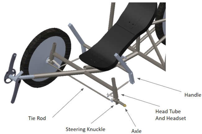
Figure 9: Full Steering Assembly
