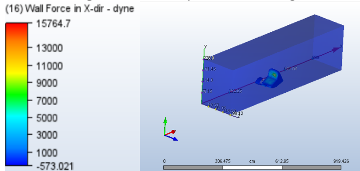
Figure 20: CFD Analysis With Fairing
