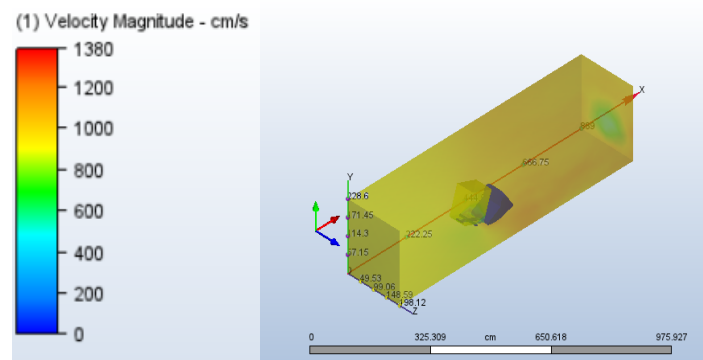
Figure 19: CFD Analysis Without Fairing
