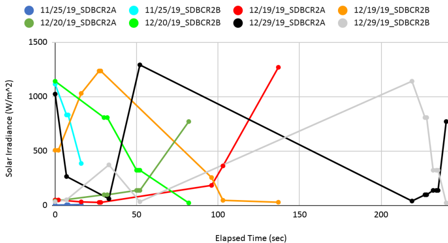
Figure 16: Solar Irradiance vs. Time (11/23/19 Night Pass)
