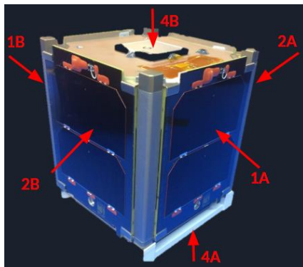
Figure 1: Diagram of Libertas detailing the naming convention of each side
