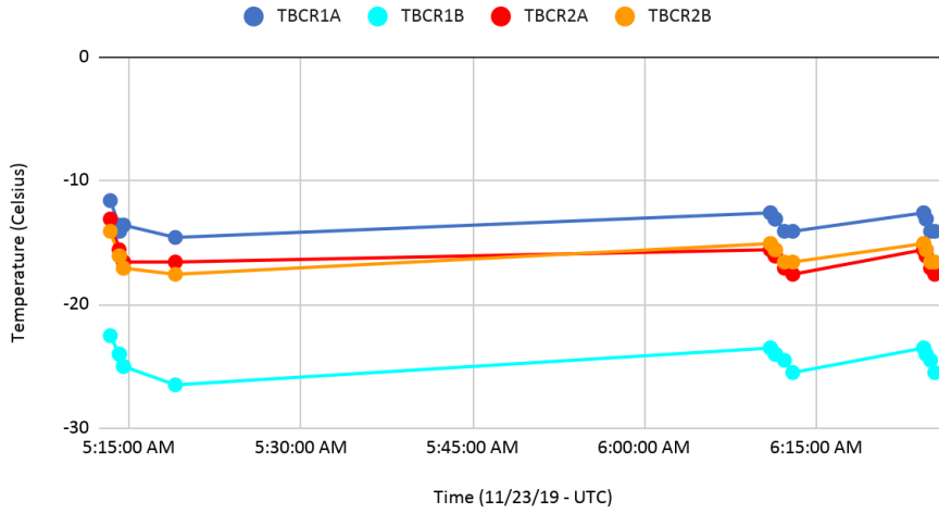
Figure 17: Temperature vs. Time (11/23/19 Night Pass)
