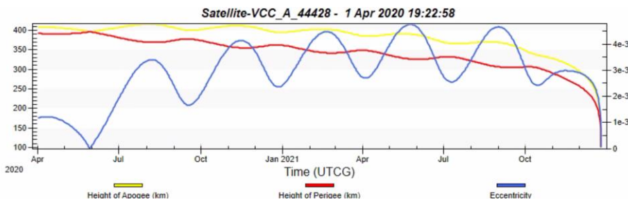
Figure 10: Deorbit prediction calculated on April 1, 2020.
