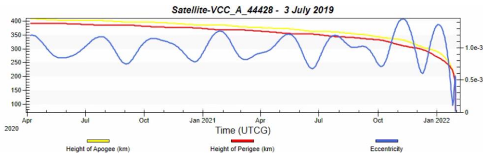
Figure 9: Deorbit status calculated on July 3, 2019
