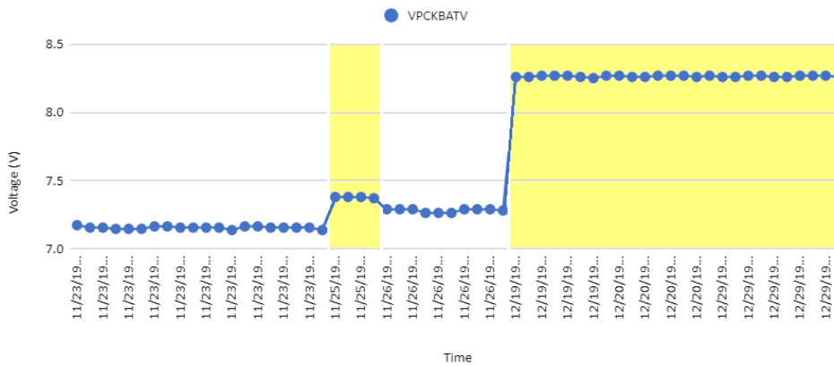
Figure 5: A Voltage vs Time plot of Libertas ' battery bus over all passes. Highlighted are the passes that occurred during the day, and non-highlighted passes represent those that occurred at night. This distinction is important in analyzing the jumps in voltages that this graph displays.
