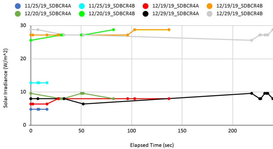
Figure 14: Solar Irradiance vs. Time - Pair 1
