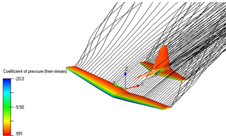
Figure 9-3. Stall Vortex Visualization
