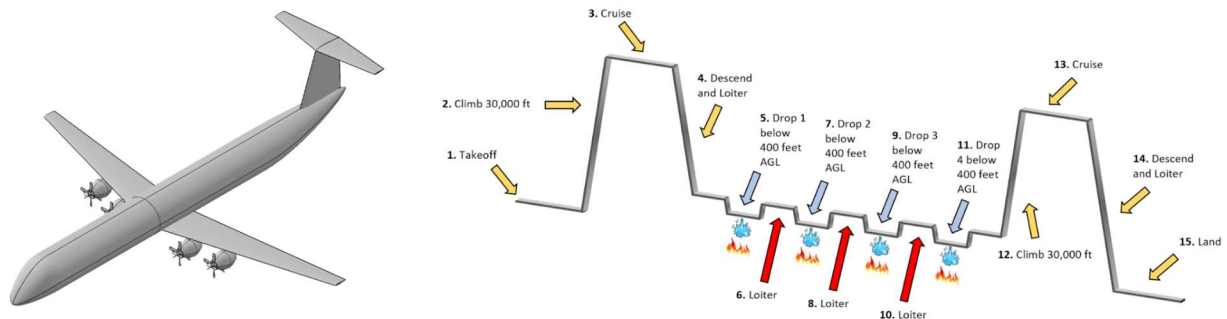
Figure 6-2. Zeus-8k Configuration and Mission Profile
