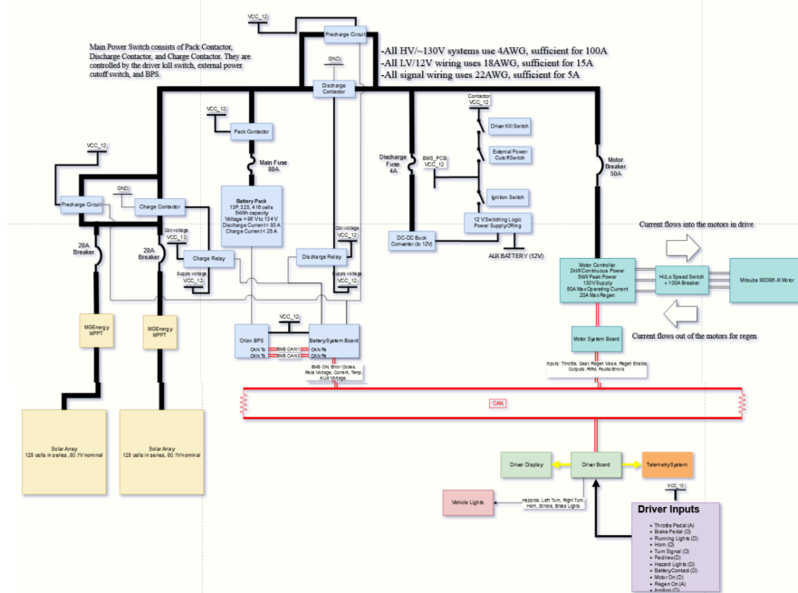
Fig. 11: Rivannna 2S Functional System Diagram
