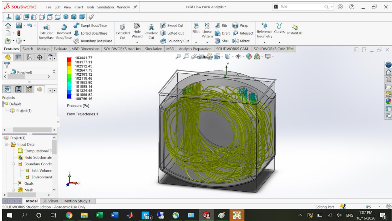
Figure 4: The initial CFD analysis performed on the fluid region.
