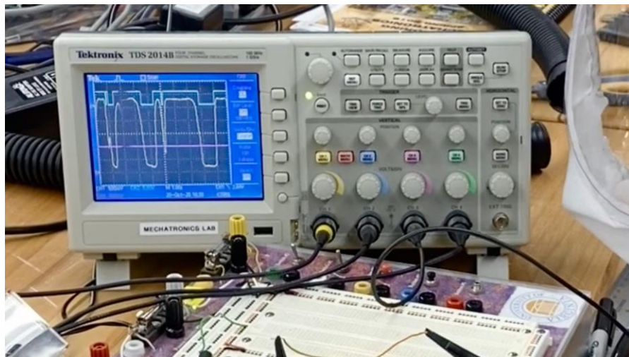
Figure 18: Oscilloscope showing the phototransistor output voltage (yellow) in relation to the threshold voltage (magenta) and the reaction of the comparator output voltage (blue).
