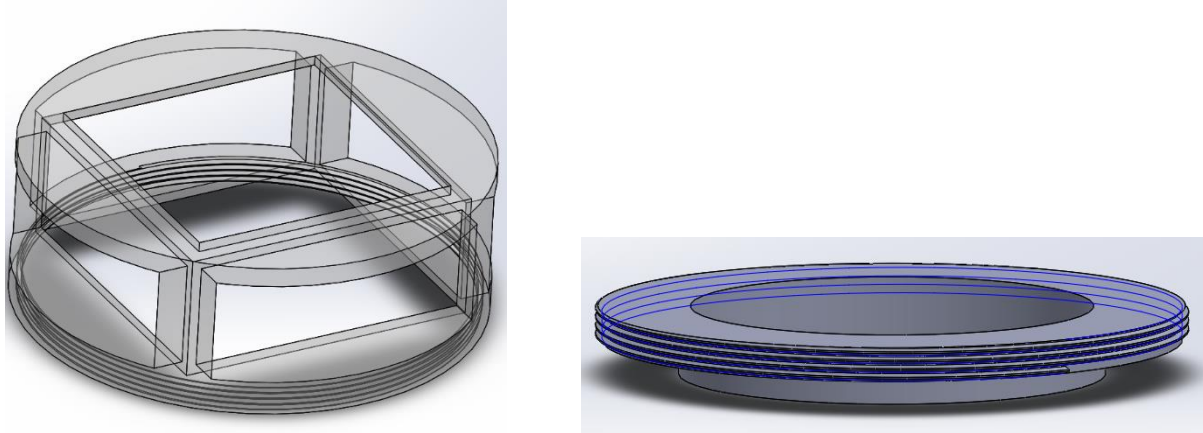
Figure 10: Second iteration of the fan casing structure.
