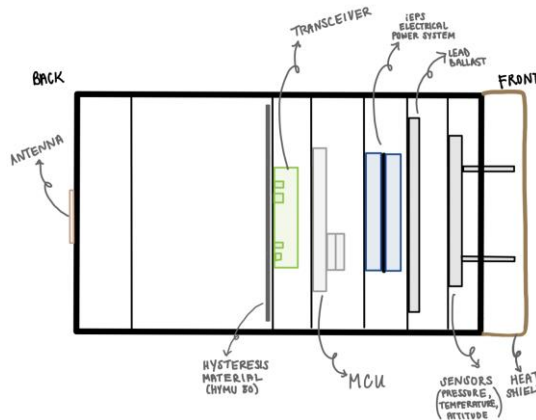
Figure 8: Internal Component Layout
