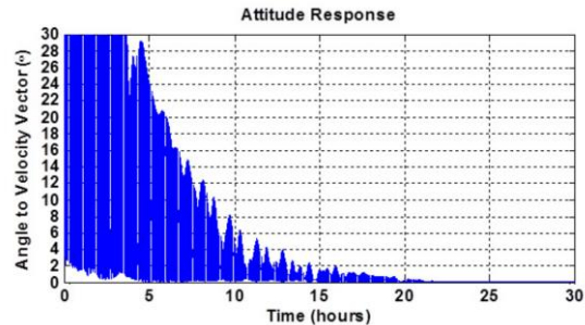
Figure 6B: Active Damping
