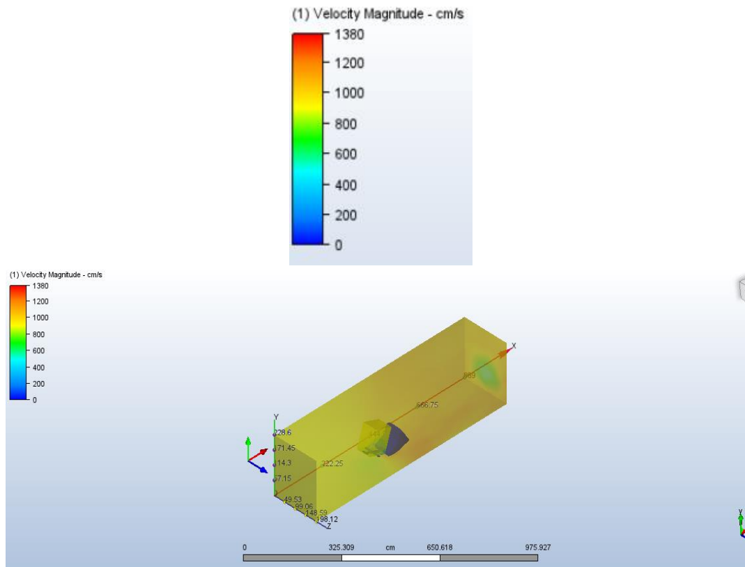
Figure 19: CFD Analysis Without Fairing
