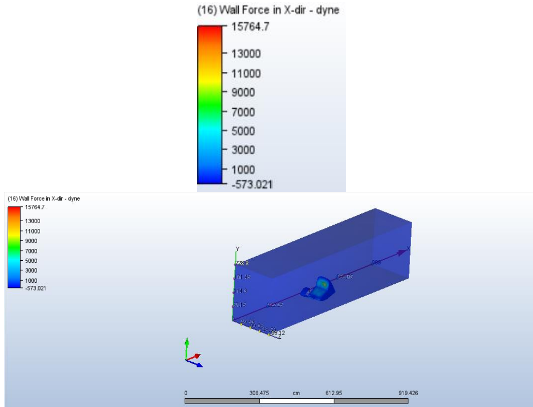
Figure 20: CFD Analysis With Fairing
