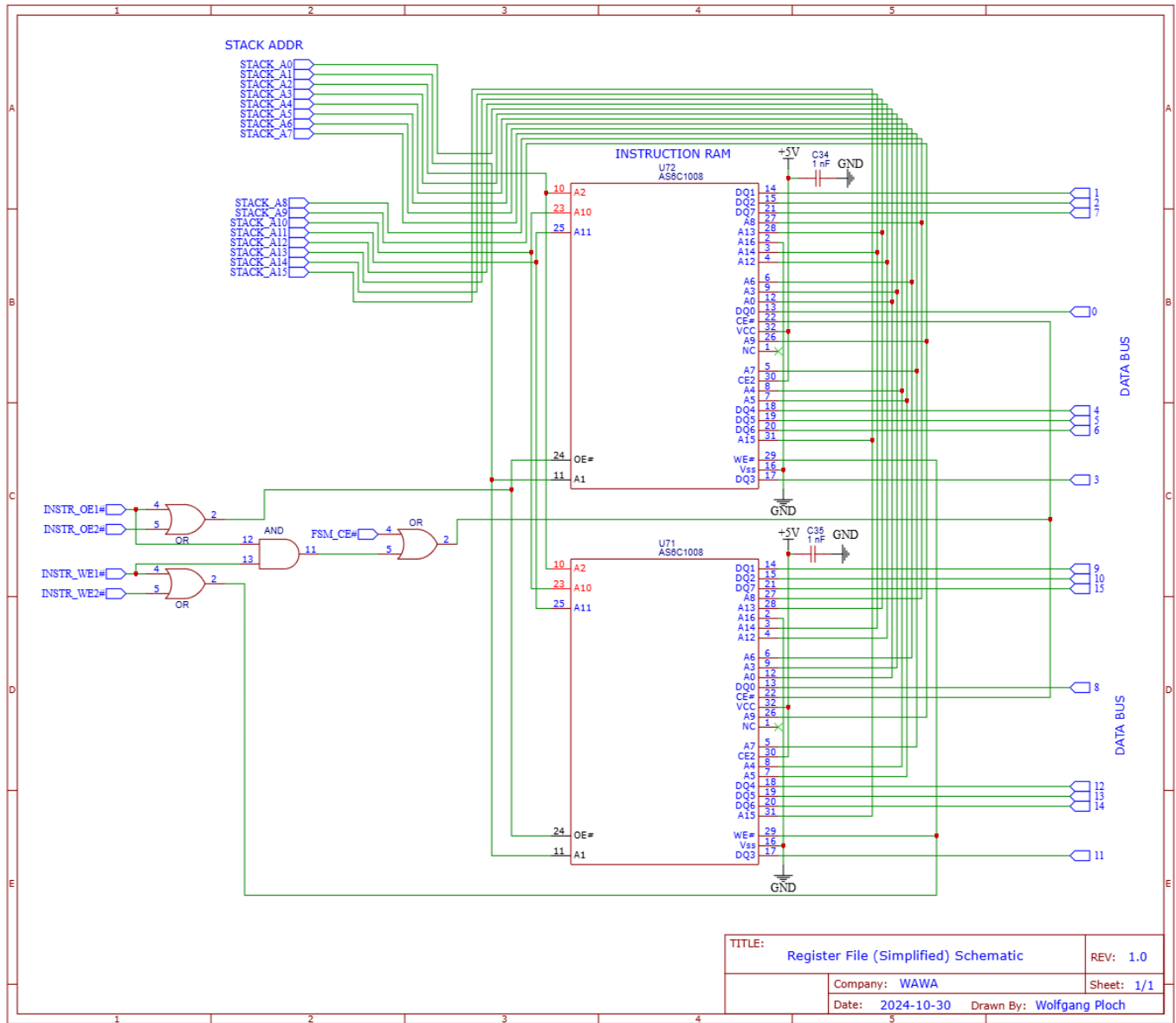
Fig. 33. Stack SRAM and Associated Circuitry
