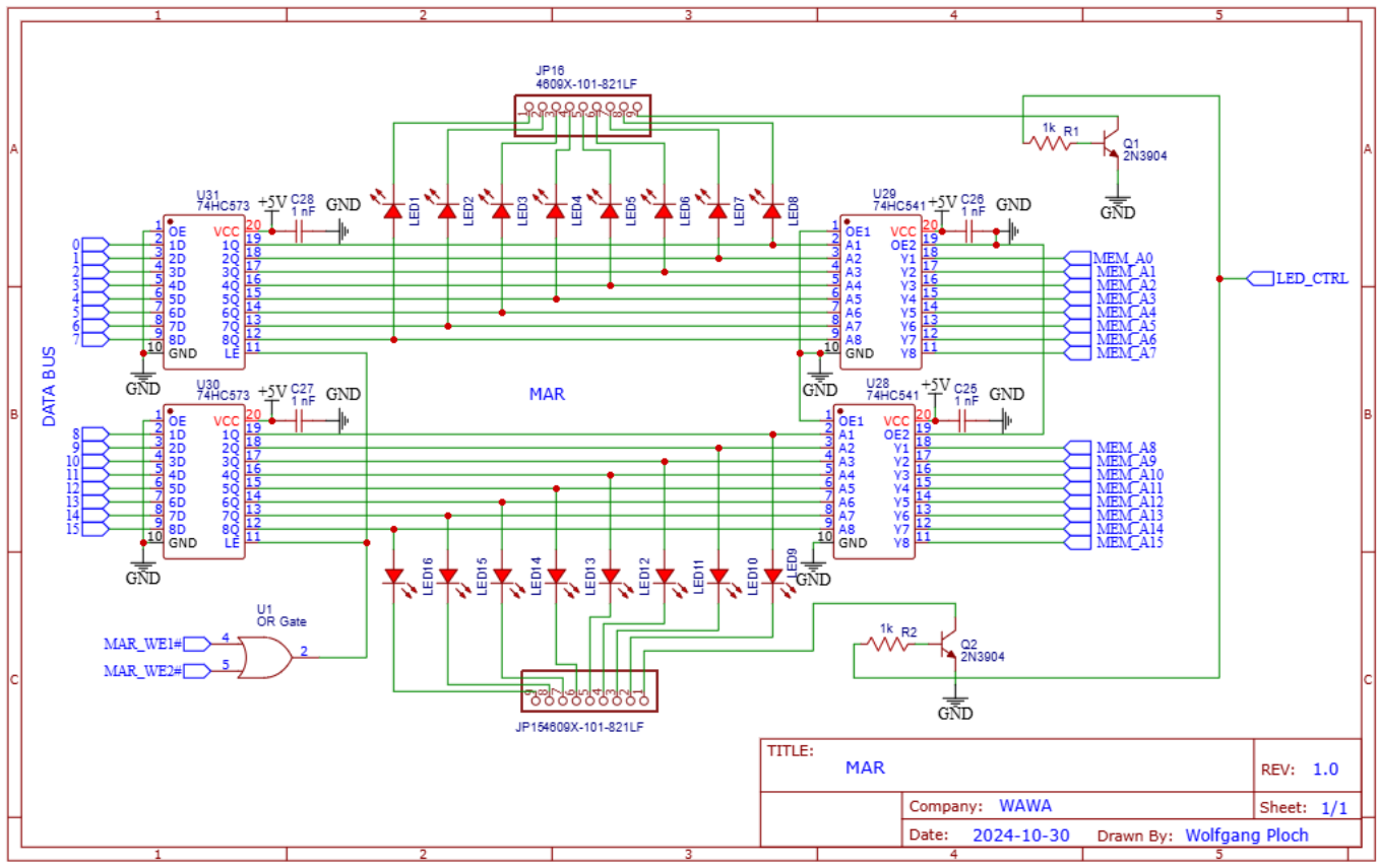
Fig. 19. Memory Address Register (MAR) Circuitry
