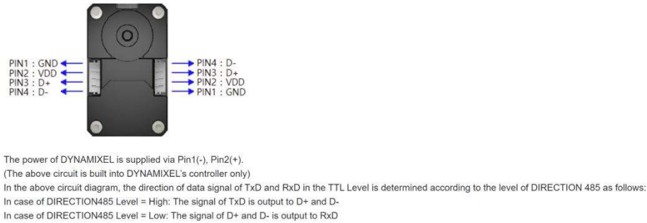
Figure 9: Dynamixel Motor Wiring Diagram
